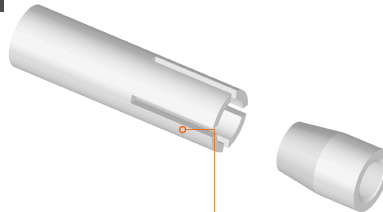
IN - 7000 - Chumbador Jaqueta e Cone
