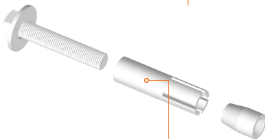
IN - 7010 - Chumbador CBC c/ Parafuso
